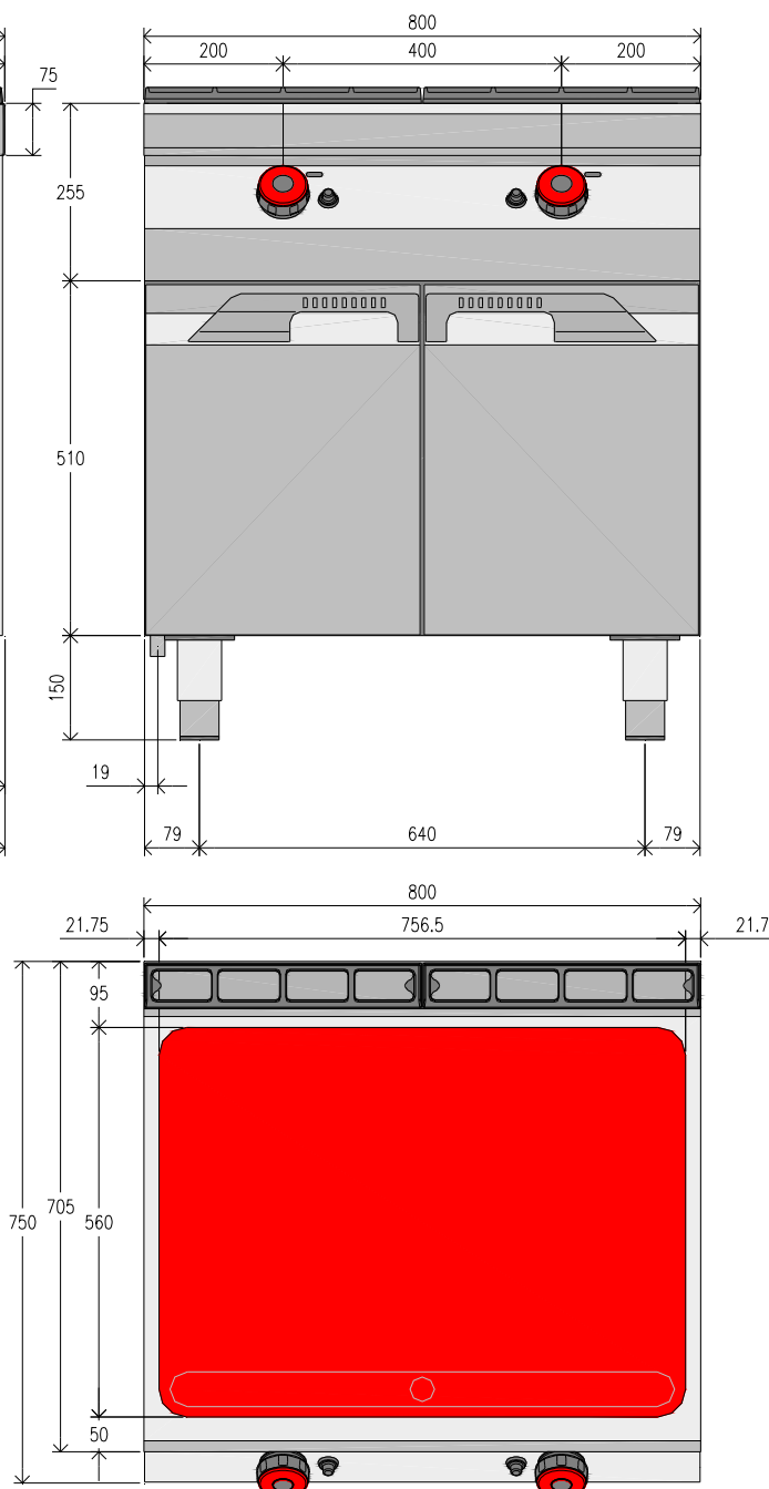
Vista frontal
