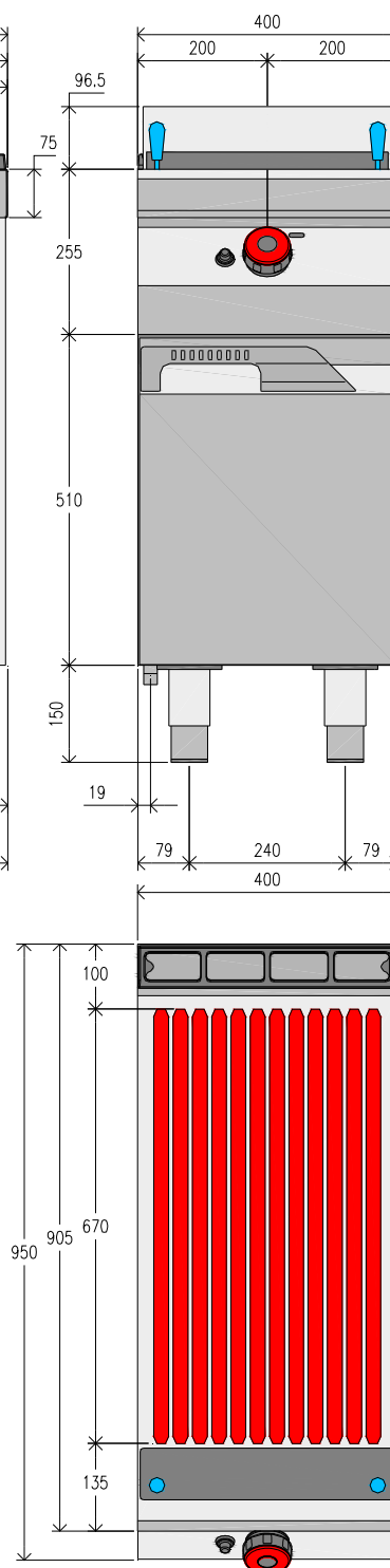
Vista frontal
