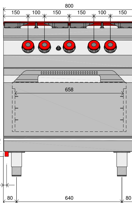
Vista frontal
